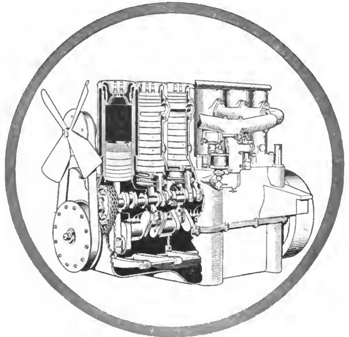
Fig. 3—Part sectional view of the Stoddard-Dayton six-cylinder Knight motor
